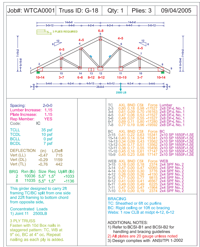
Figure 6 Truss Design Drawings
